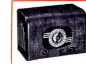
Model 54P (Code—FROM) 5 Tubes. Tunes American Broadcasts, Police, Amateurs, Aviation, and Short Wave. Electro-Dynamic Speaker; Modern Circuit; High Impedance Litz Coils; Large Scan Illuminated Airplane Dial; Self Contained Antenna. Cabinet dimensions 10 1/2 x 7 1/2 x 5". List Price.....$19.95
