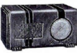
Model 4V6 (Code—VANO) 6 Tube 6 Volt Superheterodyne. All wave 3 bands tune 550-1600 K.C., 1.8 to 5.0 M.C., 5.5 to 16 M.C. Standard American Broadcast Band, All Police Bands, Amateur and Aeroplane Stations, American and Foreign Short Wave Bands, Tone Control; Automatic Volume Control; 6 1/2" P.M. Dynamic Speaker; New 6 1/2" Gold Clock Type Dial, indirectly illuminated; Rubber Cushioned Tuning Unit. Cabinet dimensions 14 1/2 x 9 1/2 x 7 1/4". List Price.....$39.95
