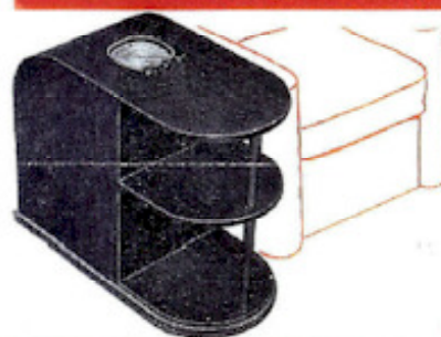
Model 7165Q (Code—TRIN) 7 Tubes. 2 1/2 Bands Tunes 550 to 1700 K.C.—2.4 M.C. to 7 M.C. American, Foreign, Police, Amateurs, Aviation, Ships at Sea. Electric Tuning Eye; Automatic Volume Control; Rubber Cushioned Tuning Assembly; 6 1/2" Full Tone Oversize Dynamic Speaker. Cabinet dimensions 14 1/2 x 9 1/2 x 7 1/4". List Price.....$34.50
