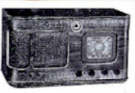
Model 7165Q (Code—TRIN) 7 Tubes. 2 1/2 Bands Tunes 550 to 1700 K.C.—2.4 M.C. to 7 M.C. American, Foreign, Police, Amateurs, Aviation, Ships at Sea. Electric Tuning Eye; Automatic Volume Control; Rubber Cushioned Tuning Assembly; 6 1/2" Full Tone Oversize Dynamic Speaker. Cabinet dimensions 14 1/2 x 9 1/2 x 7 1/4". List Price.....$34.50
